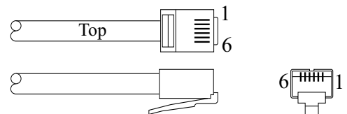
Pin Configuration RJ-12 Plug
